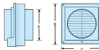
Dimensions SF150/ID150 Series
