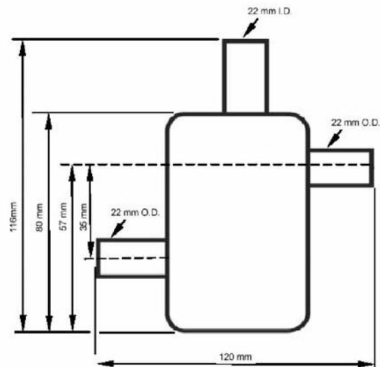
22mm air separator dimensions
